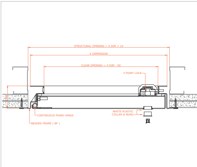
Non-fire rated, beaded frame, metal door, 3 point lock, single door 4000-NFR-BF-MD-3PC-SD
