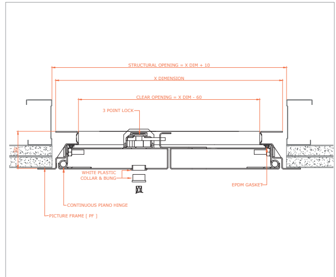
Non fire rated, picture frame, metal door, 3 point lock, double door, EPDM gasket 4000-NFR-PF-MD-3PL-DD-EPDM
