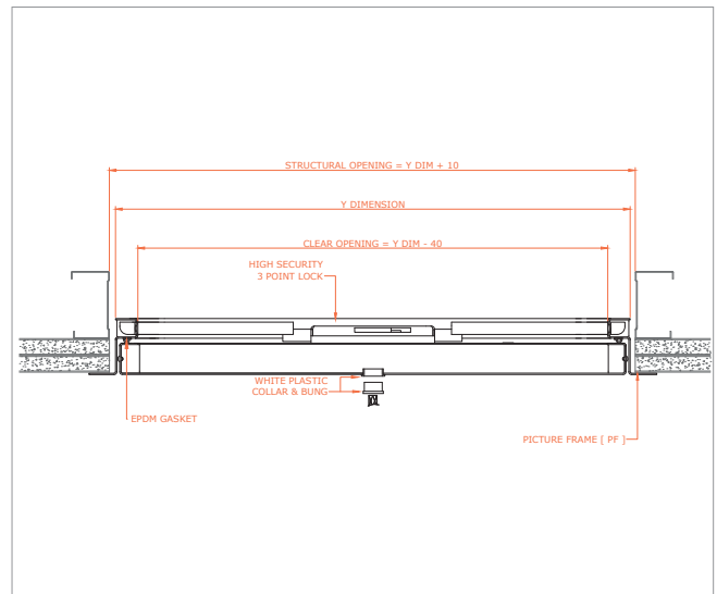
Non fire rated, picture frame, metal door, 3 point high security lock, single door, EPDM gasket 4000-NFR-PF-MD-3HS-SD-EPDM
