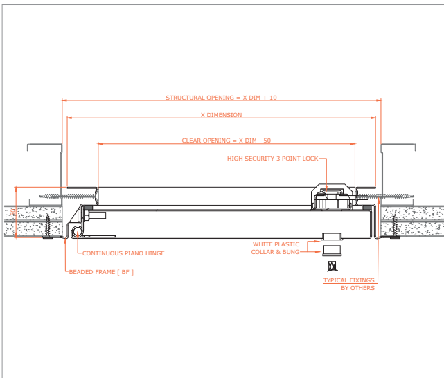
Non fire rated, beaded frame, metal door, 3 point high security lock, single door 4000-NFR-BF-MD-3HS-SD
