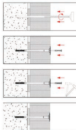
Anchor installation for all insulation types
