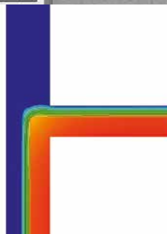
Efficient solution with Schöck Isokorb® XT Type A.
