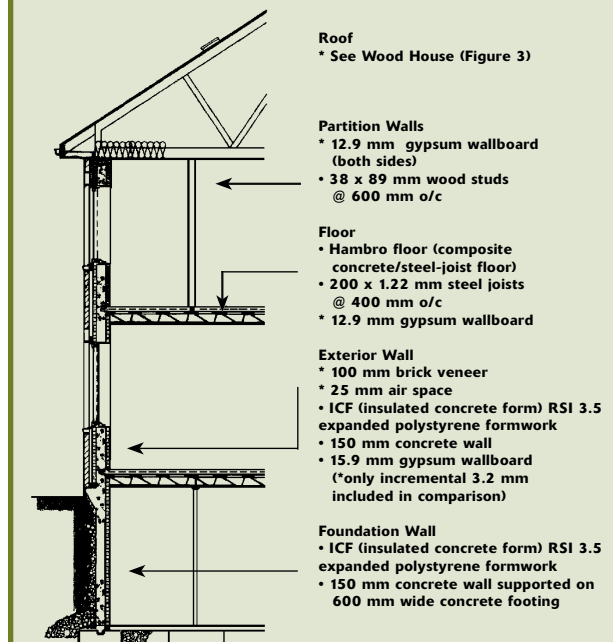
FIGURE 5: Concrete House Cross-section
