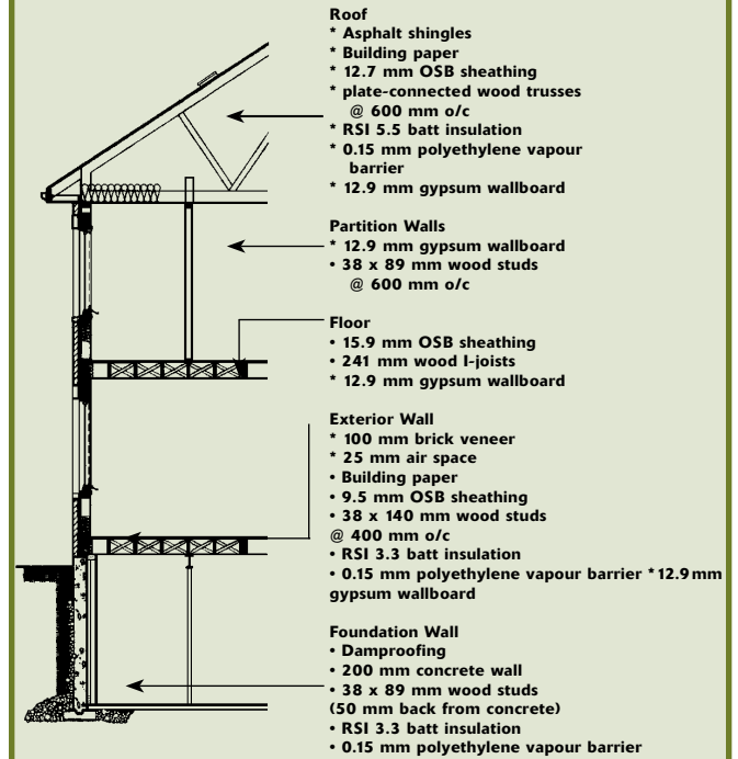
FIGURE 3: Wood House Cross-section
