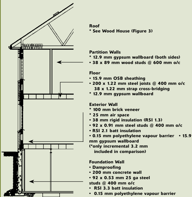
FIGURE 4: Sheet Metal House Cross-section
