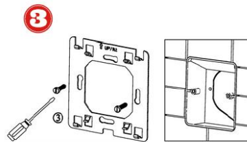
Install the thermostat into the electrical connection box with screws
