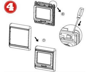
Install the housing cover and lock the external frame
