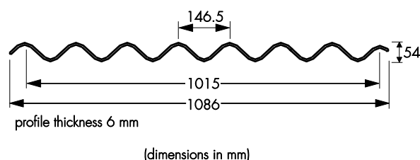
Figure 1 Cemsix — profile and dimensions
