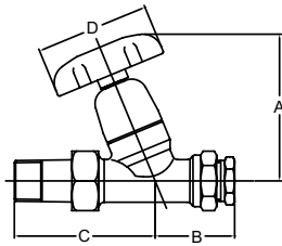
15mm & 1/2" Straight (for horizontal mounting)
