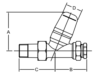
15mm & 1/2" Straight (for horizontal mounting)
