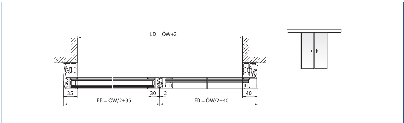
2-leaf door system
