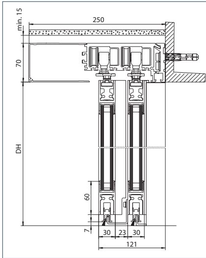
Drawing no. 70487-ep01
