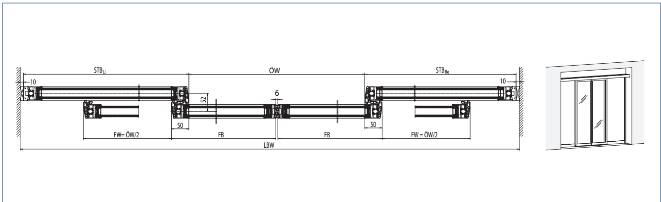
2-leaf , horizontal section
