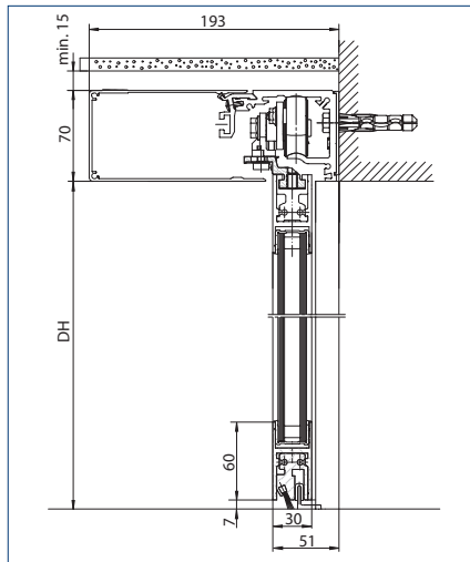
Drawing no. 70511-ep01
