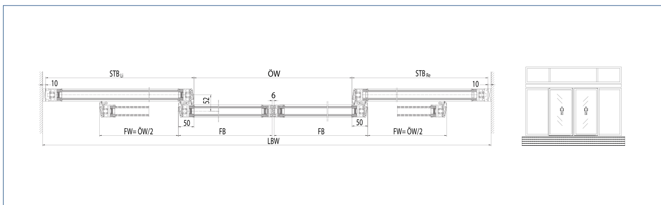
Horizontal section
