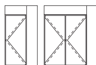
Compositions with fixed light
