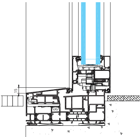
Vertical cross-section - opening sash, build-in threshold
