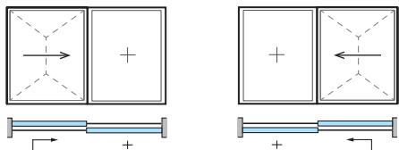
1 leaf + fixed
