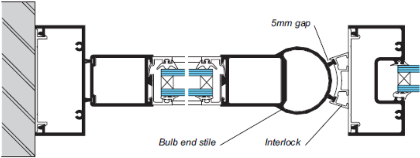
Pivot door featuring anti-finger-trap stile. (Scale 1:3)
