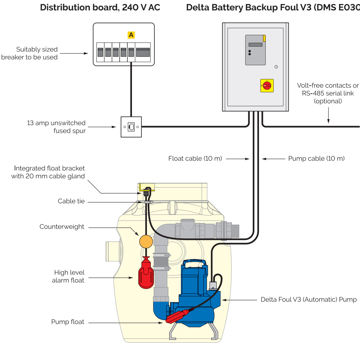
Delta Foul V3 packaged pumping station (DMS 165)
