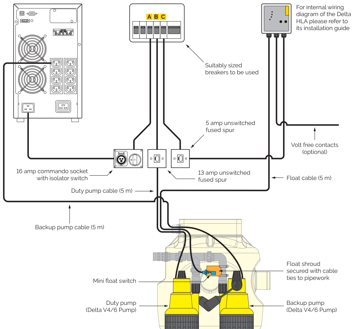
Delta Dual V4/6 packaged pumping station (DMS 217/079)
