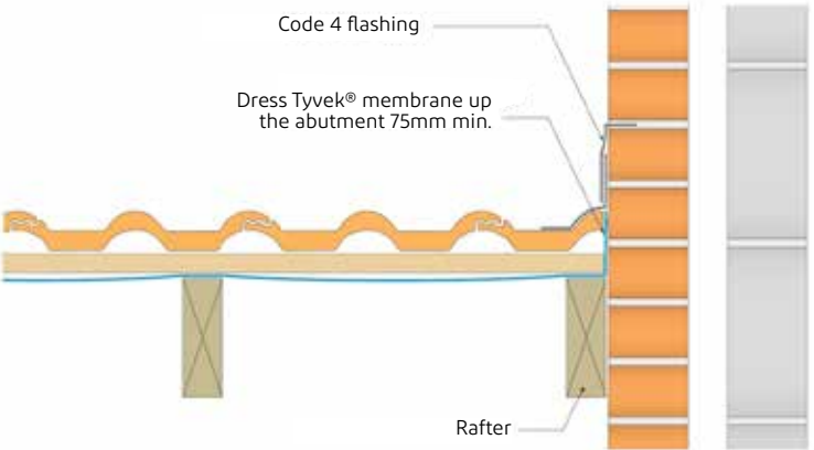
Fig. 43 - Abutment
