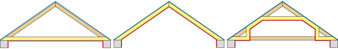
Fig. 5 - Cold roof
