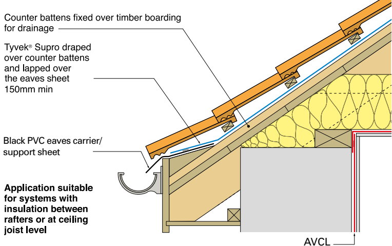
Fig. 32 - Membrane unsupported over timber sarking
