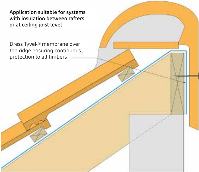
Fig. 41 - Mono-pitch ridge
