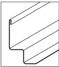
Wall W-profile Fe 0.6 mm Alu 0.8 mm (45 x 21 x 21 x 18.5)
