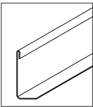
Wall L-profile Fe 0.6 mm Alu 0.8 mm (45 x 18.5)
