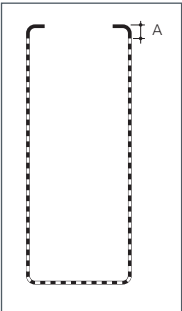
D1522, full perfo A = 10 mm
