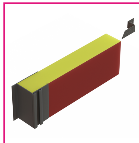
Thermo-loc FR60+ Profile and Fixing Flange
