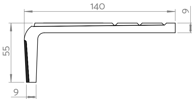
Fig 1. Side view of SN93/SL3/140 stair nosing.
