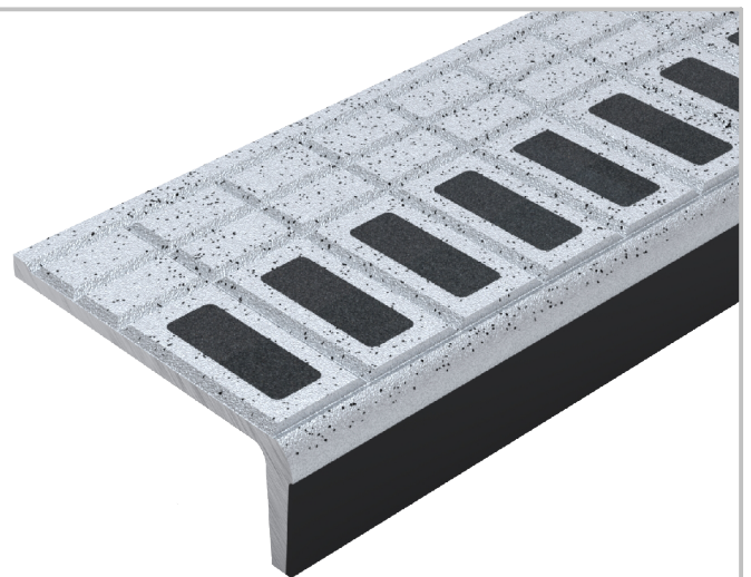
Fig 3. 3D view SN93/SL3/140 stair nosing.
