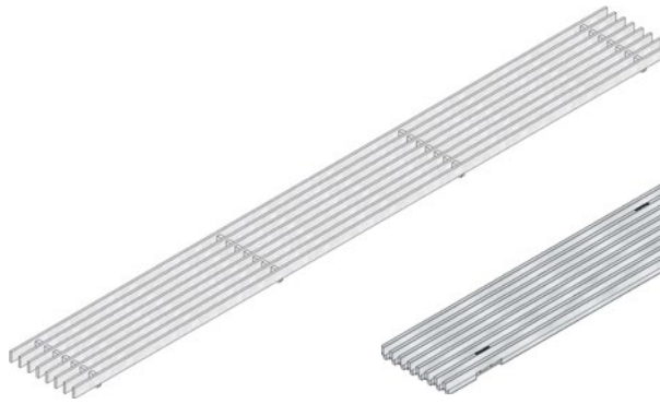
Longitudinal grating SW 12 mm, 1,0 m
