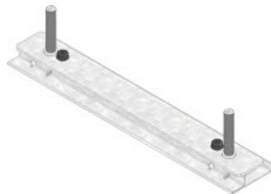
Height adjusting set DACHFIX STEEL 255, type 75, 100, 150, galvanised (2 pieces per metre required)
