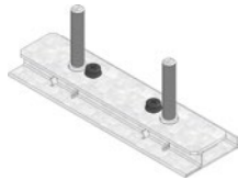
Height adjusting set DACHFIX STEEL 155, type 75, 100, 150 galvanised (2 pieces per metre required)
