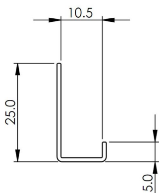
End Cap Profile
