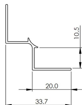
Internal Corner Profile
