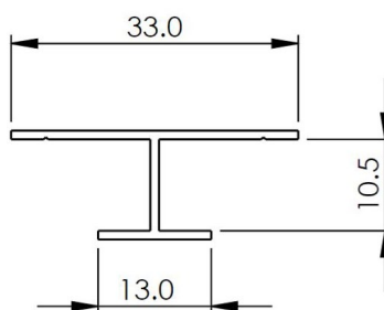
H-Section Profile
