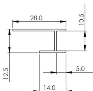
Bottom/Top Profile
