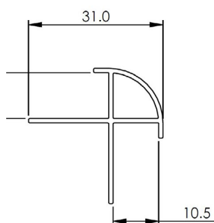
External Corner Profile
