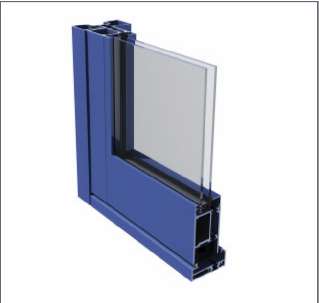
AA®190 TB Butt Hinge and Rebated Threshold Open Out (external view)
