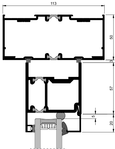
Head Detail
