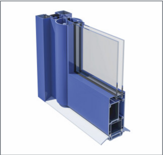
AA®190 TB Round Finger Guard with Threshold (internal view)
