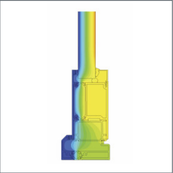
Butt Hung Open In Threshold
