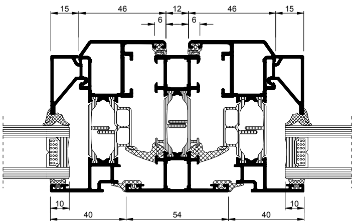
JAMB DETAIL (TILTURN NEXT TO FIXED LIGHT)
