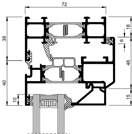
HEAD AND CILL DETAILS
