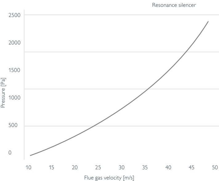
Pressure drop Resonance silencer Ø100-600
