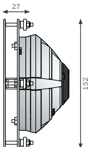
Dimensions (mm): Beam Receiver (with Parallel Bracket*)
