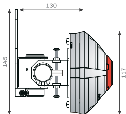
Dimensions (mm): Beam Transmitter (with Angle Bracket*)
