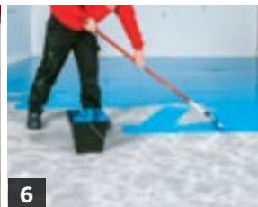
6 Apply two top coats of Fastcoat by roller
