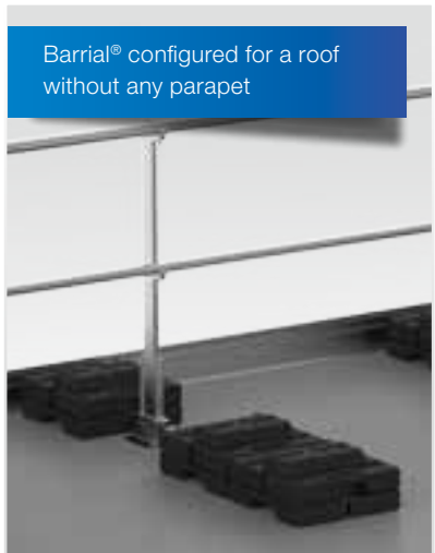
The free-standing variant can be used in special cases, including in the absence of an parapet at all.
