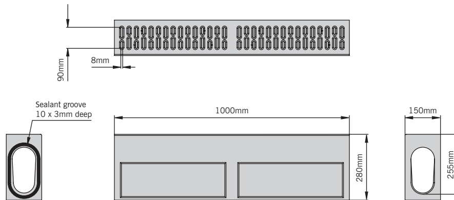
HB405 half battered flush drainable centre stone
