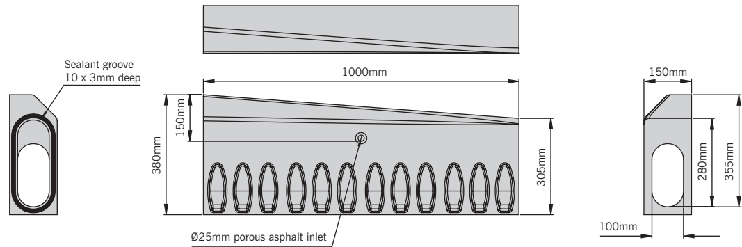
SP380 left-hand drop kerb
