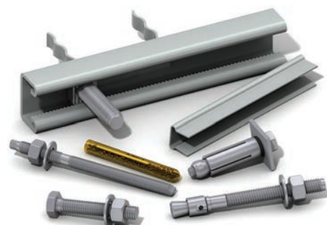
Channel & Bolt Fixings
