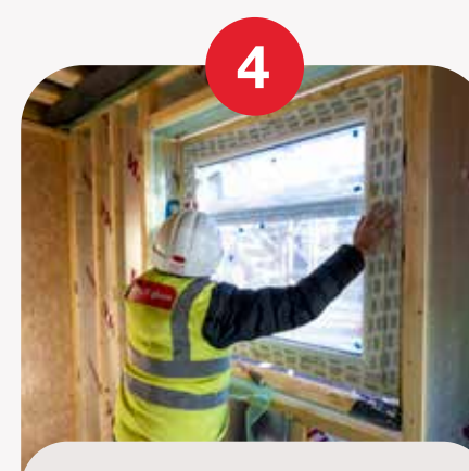
4 LOCK INSITE INTO POSITION (PUSH-OUT)
