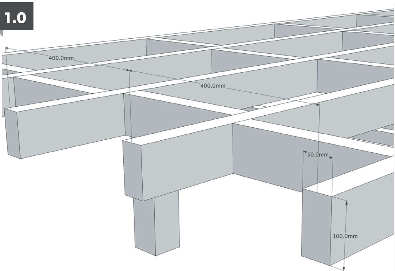
Typical timber sub-frame
