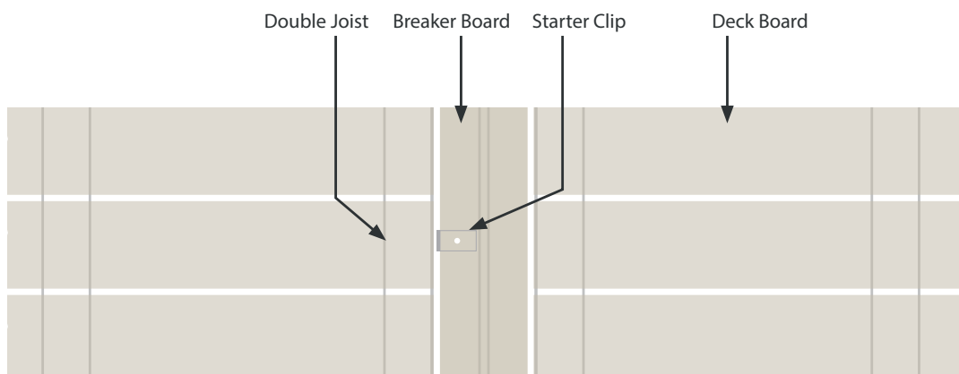
Breaker Board - Starter Clip - Plan View
