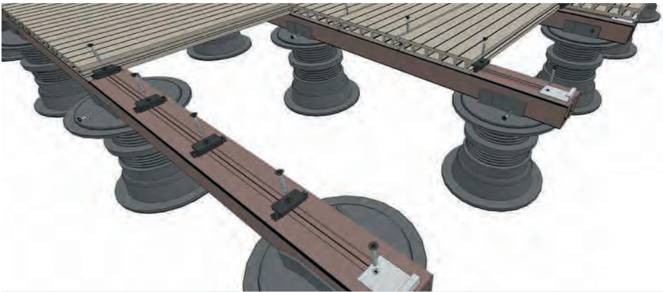
Typical aluminium / plastic sub-frame on adjustable pedestals
