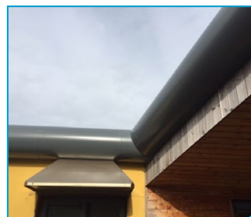
Anti-Climb
