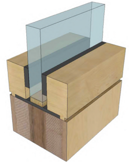
F6 Profile
