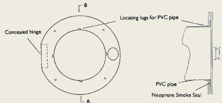
TYPICAL HINGEPLATE DETAIL FOR WALLS AND CEILINGS
