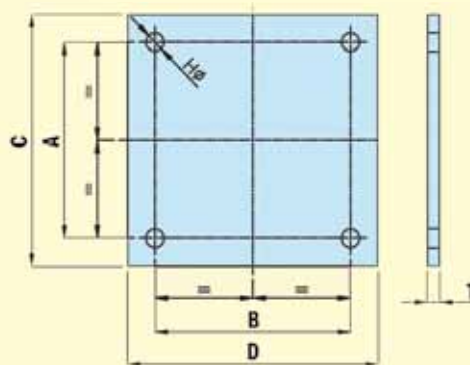
Location Plate Dimensions for Type BY
