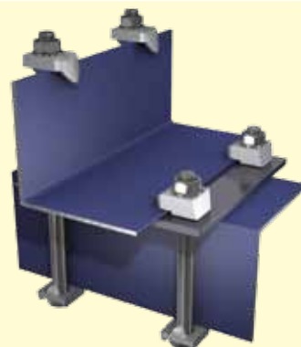
Angle section to another angle section at 90 degrees
