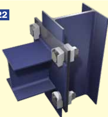
I-Section to I-Section column using a location plate
