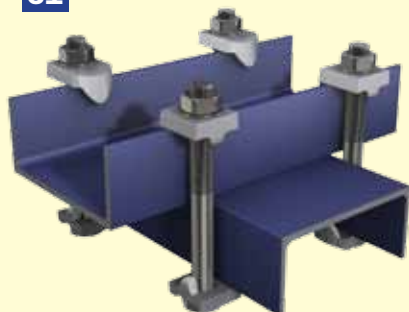
Two channels secured back to back
