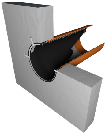
Clamp mounting edge inside a manhole
