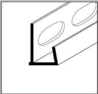
PE12 PE15 Clip-on plasterboard or render carrier board edge bead providing reinforcement
