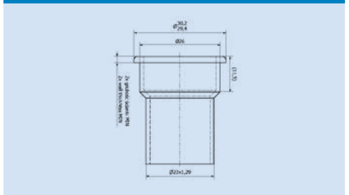
End Forming
