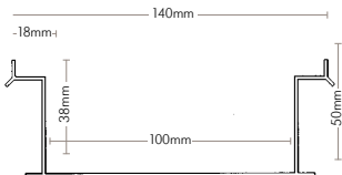
Dimensions of the Type I in-screed services duct.
