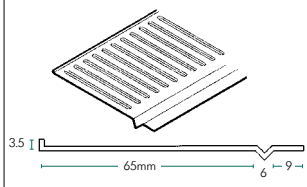
Profile and dimensions of SV-FL
