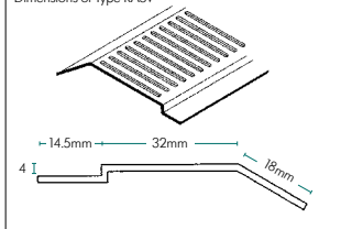
Dimensions of Type RASV
