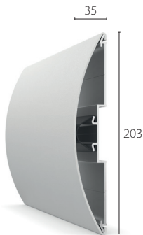
Continuous retainer Heavy Duty
