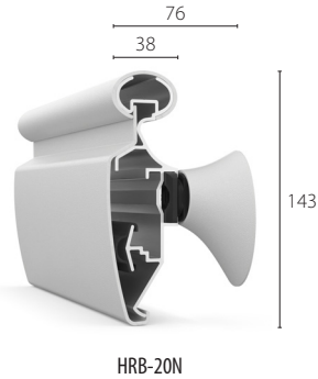
Quick Lock bracket
