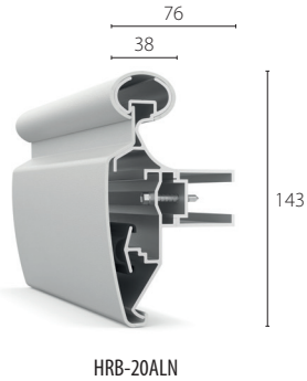
Anti-ligature bracket
