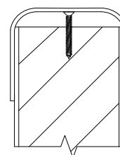
Overlapping door face protection
