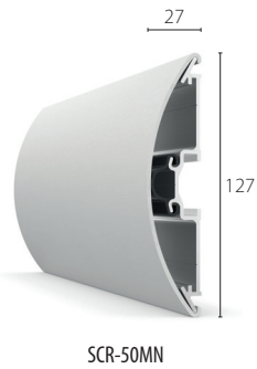
Continuous retainer Heavy Duty
