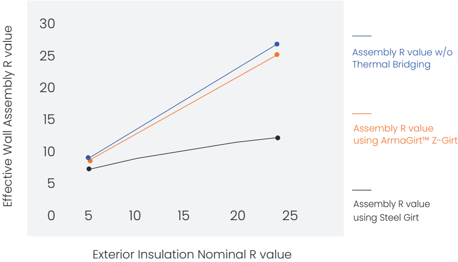
EFFECTIVE WALL ASSEMBLY R VALUE COMPARISON WITH HORIZONTAL GIRTS AT 24" SPACING
