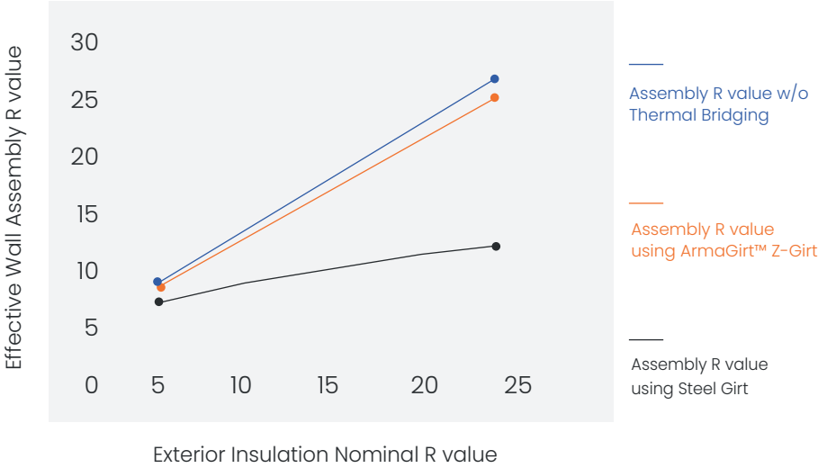
EFFECTIVE WALL ASSEMBLY R VALUE COMPARISON WITH VERTICAL GIRTS AT 16" SPACING
