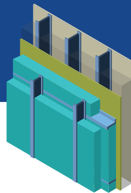
VERTICAL & HORIZONTAL ARMAGIRT™ Z-GIRT
