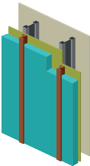
Wall assembly using vertical ArmaGirt™ Z-Girt
