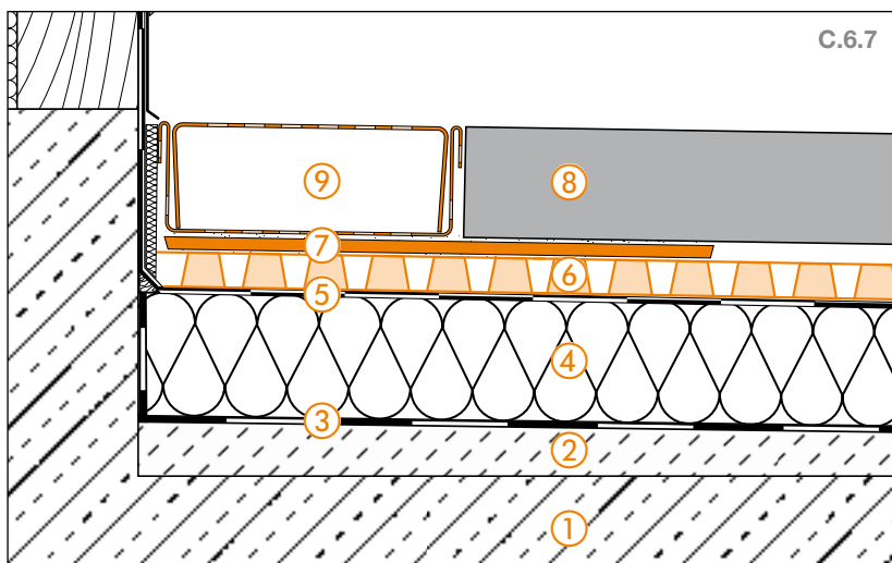
Threshold
