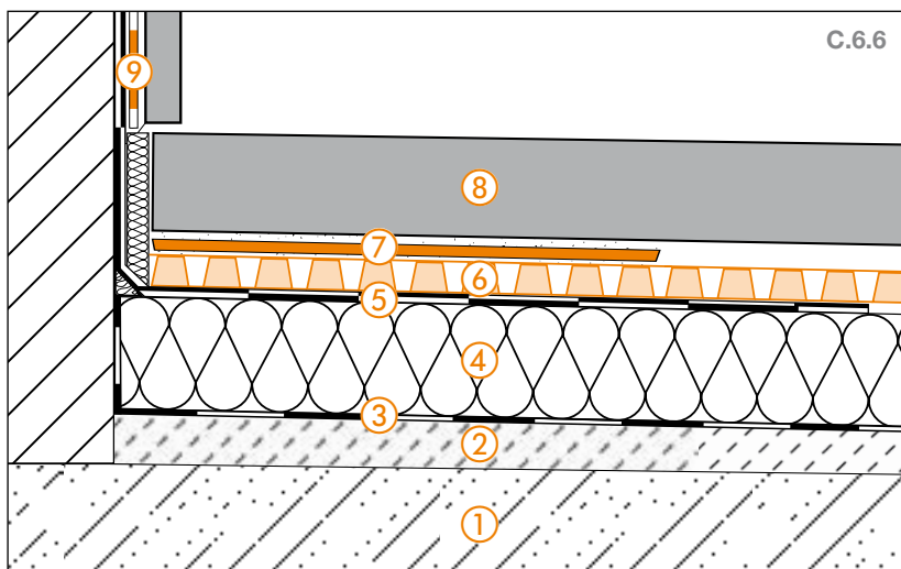
Wall transition
