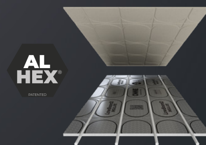
EPS Floor Deck Panel with AL HEX foil diffuser
