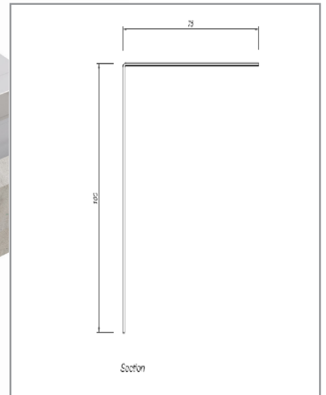
Tortrim HE - Hard Edge 75mm
