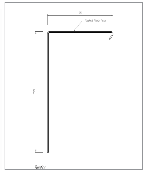
Tortrim 130D - Drip Trim
