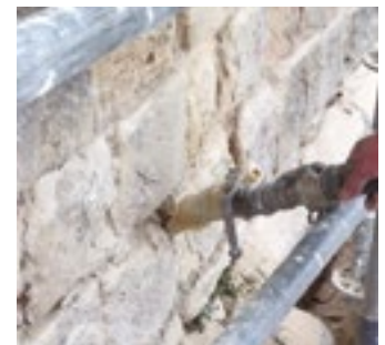
Consolidation of “rubble masonry” stone masonry
