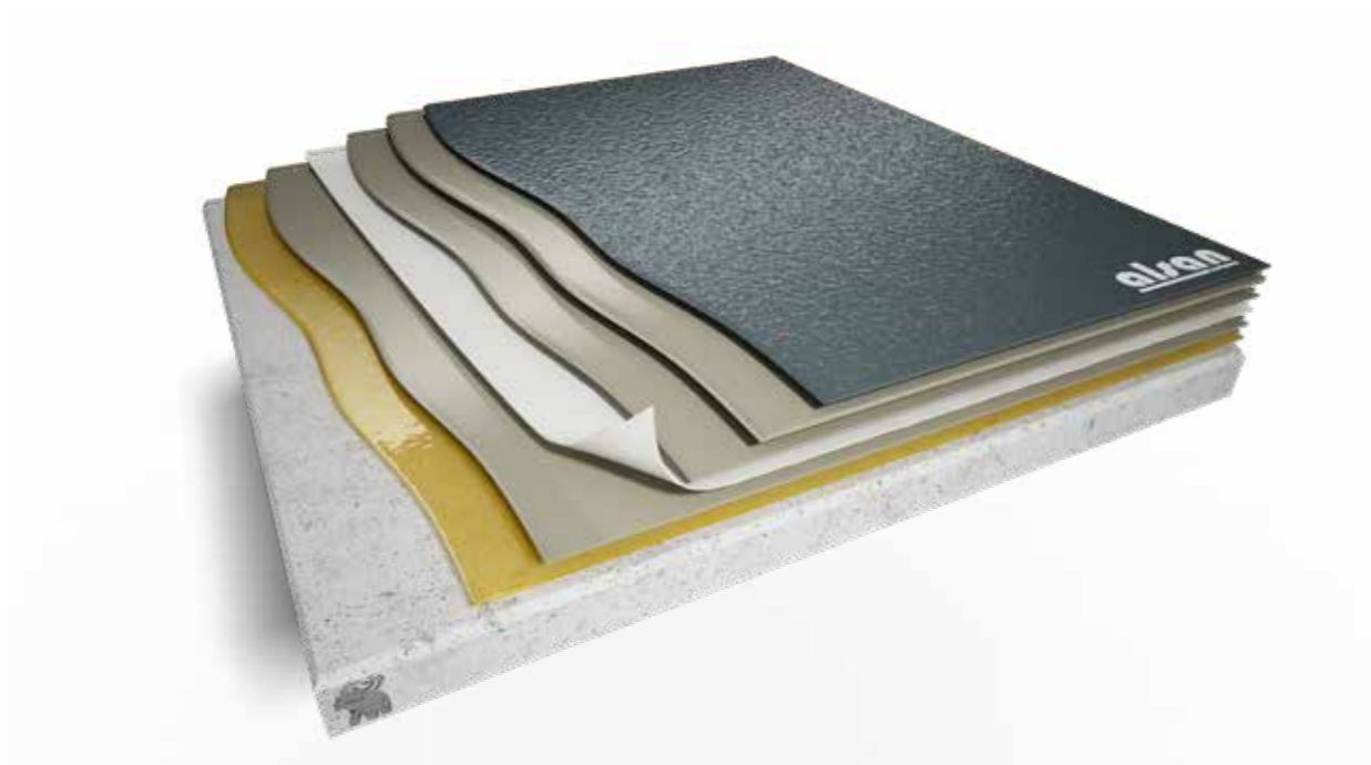
ALSAN® 770.04 THICK REINFORCED STRUCTURED WATERPROOFING SYSTEM
