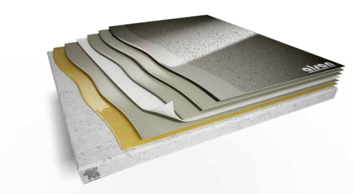
ALSAN® 770.01 DECORATIVE WATERPROOFING SYSTEM
