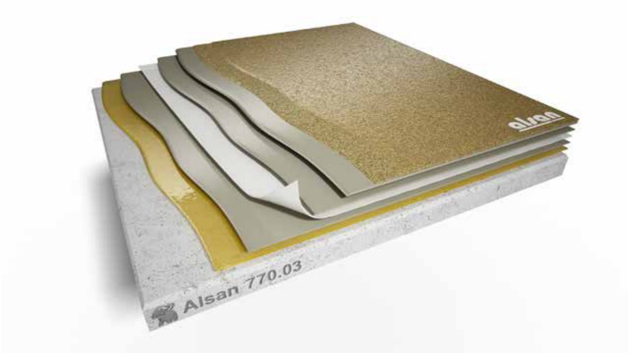
ALSAN® 770.03 NON SLIP AESTHETIC REINFORCED WATERPROOFING SYSTEM
