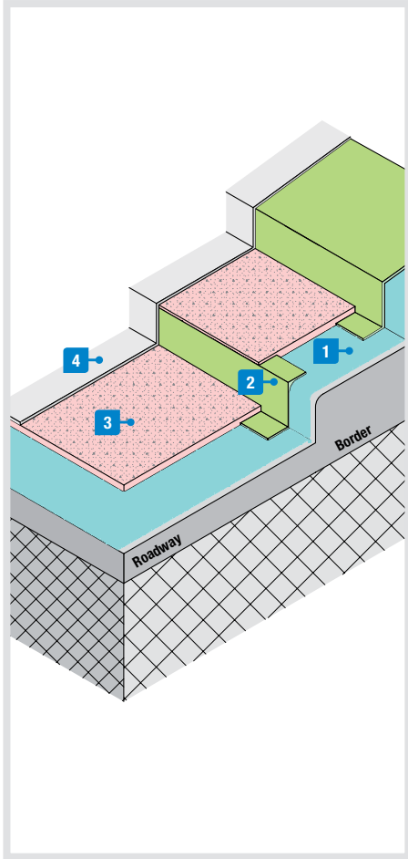
TRAFFICABLE CONCRETE RAMP JOINT
