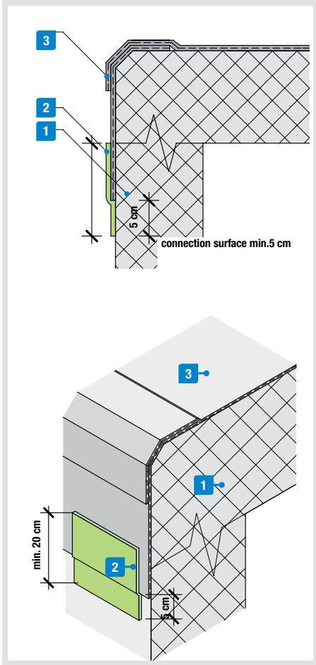
UNDERGROUND EDGE DRIP DETAIL FOR BITUMINOUS WATERPROOFING
