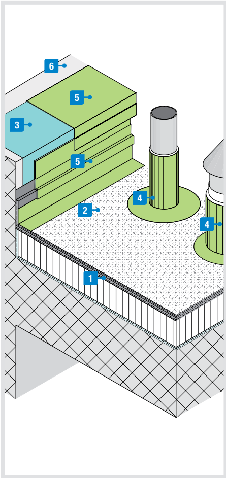
ACROTERION JOINT
