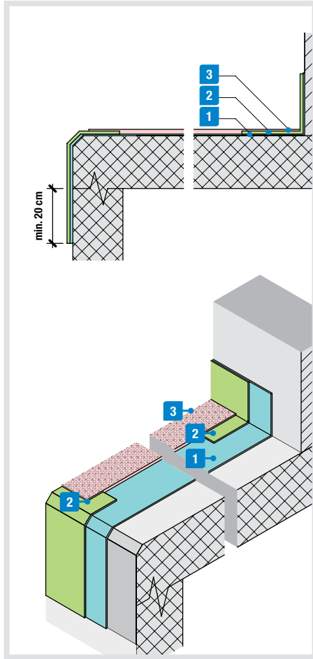
WATERPROOFING OF UPSTANDS AND EDGE DRIP DETAILS
