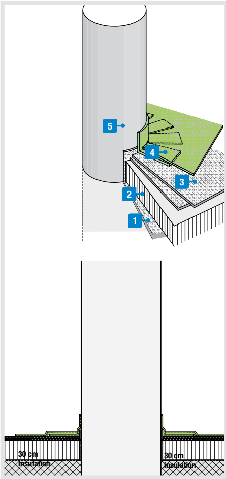
DRAIN/PIPE PENETRATIONS
