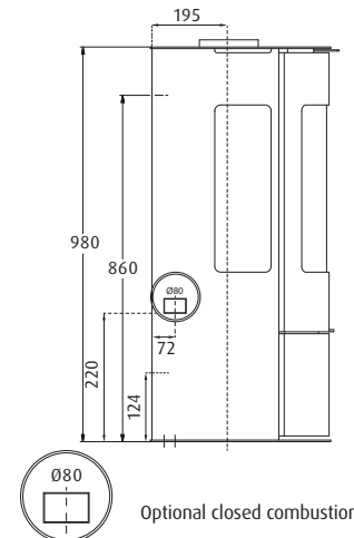
WESTFIRE.UNIQ.36 WESTFIRE.UNIQ.37 WEIGHT: 90 KG
