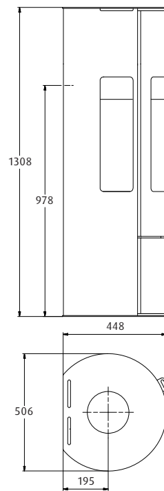
WESTFIRE.UNIQ.45 WITH BOTTOM DOOR WEIGHT: 90 KG
