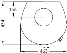
WESTFIRE.UNIQ.35 | 50 MM BLOCK WEIGHT: 95 KG
