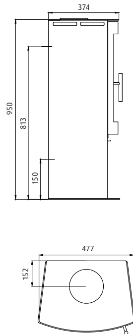
WESTFIRE.UNIQ.45 WEIGHT: 90 KG
