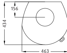
WESTFIRE.UNIQ.35 | INSERT 4-SIDED FRAME WEIGHT: 75 KG
