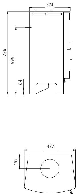
WESTFIRE.UNIQ.44 WEIGHT: 82 KG
