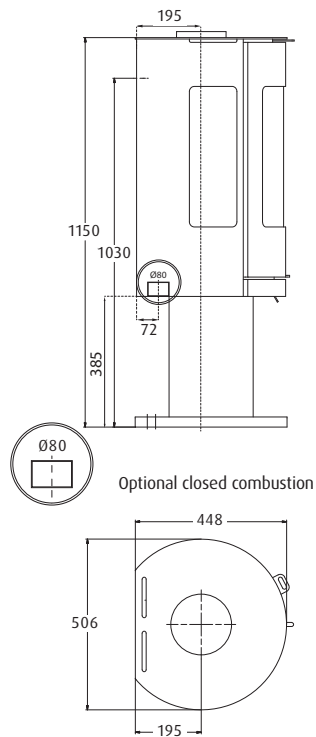
WESTFIRE.UNIQ.36 WESTFIRE.UNIQ.37 PEDESTAL 1 | WEIGHT: 95 KG
