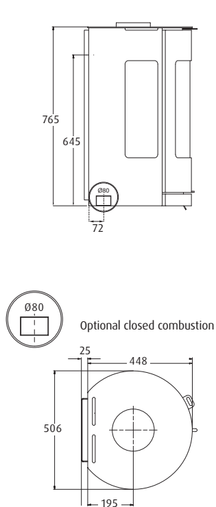
WESTFIRE.UNIQ.36 WESTFIRE.UNIQ.37 WALL-MOUNTED | WEIGHT: 85 KG
