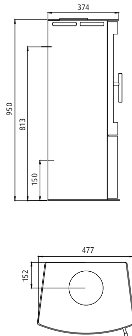
WESTFIRE.UNIQ.45 WITH BOTTOM DOOR WEIGHT: 90 KG
