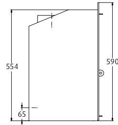
WESTFIRE.UNIQ.35 | INSERT 3-SIDED FRAME WEIGHT: 75 KG
