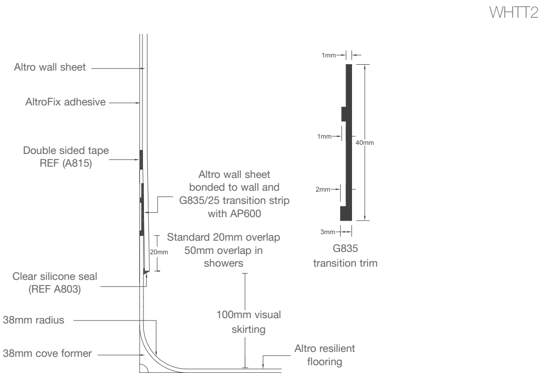
Concealed transition strip
