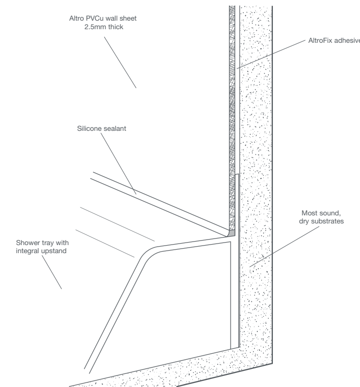
Altro Whiterock hygienic PVCu wall system to shower tray with integral upstand detail
