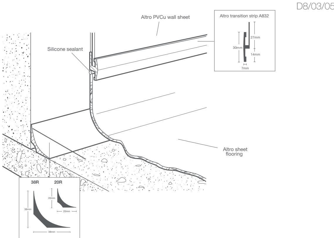
Self-coved with cove former to Altro wall system semi-rigid PVCu sheet
