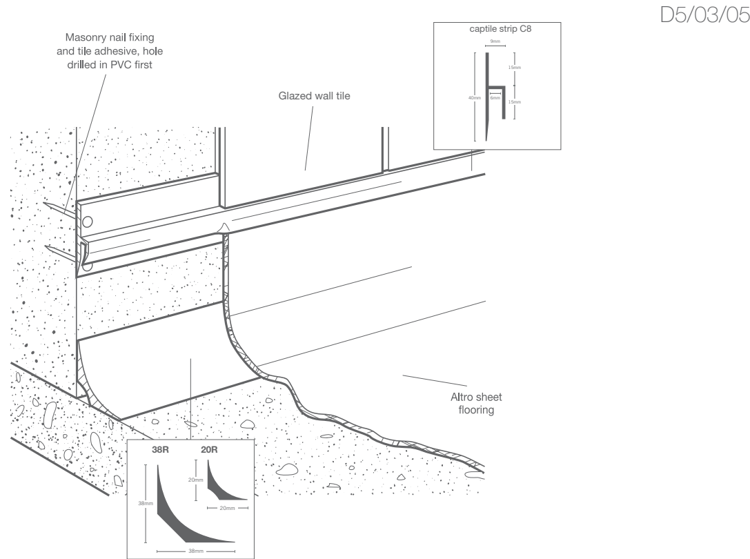
Self-coved with cove former and captile strip C8 to wall tiles
