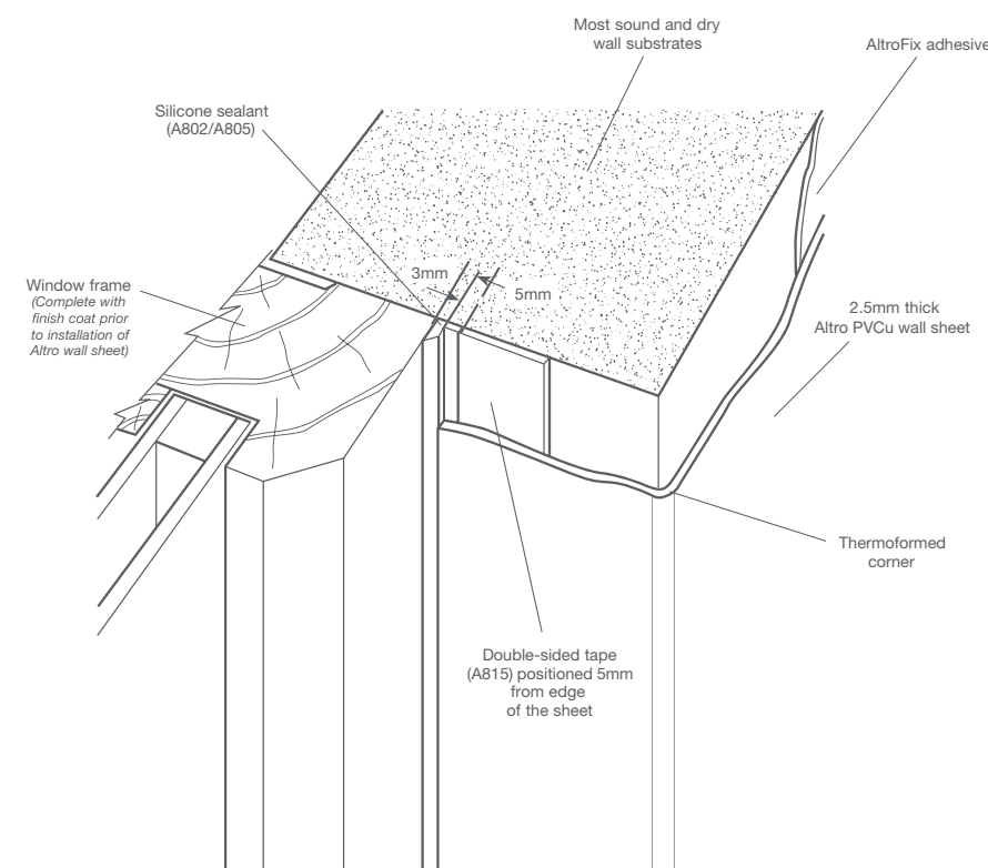
Altro wall system to window / door frame detail
