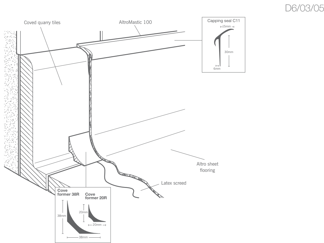
Self-coved with cove former and capping seal C11 over floor tiles
