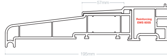
150mm A type cill AC 150
