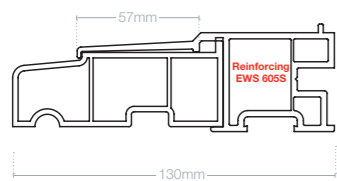
85mm A type cill AS 85
