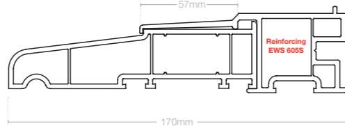
125mm A type cill AC 125
