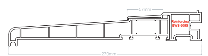
225mm A type cill AC 225
