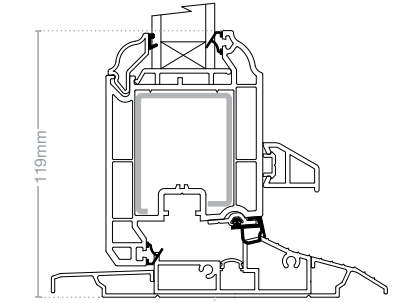
Low threshold assembly EWS 7545A and EWS 7546A
